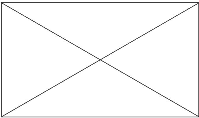
Mediand and altitudes
